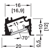
[Routing dimensions]
