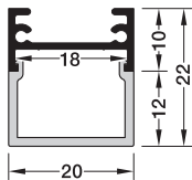
Surface mounted diffuser
