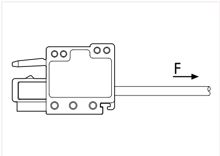
Test Arrangement per UL 1059, UL 486 E:
