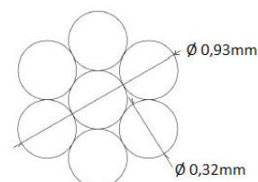
Sealing Wire Dimensions
