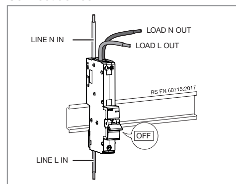
Fig 4: Connect the RCBO-AFDD
