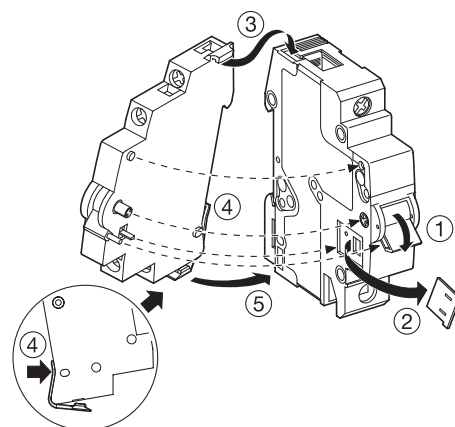
Auxiliary contact
