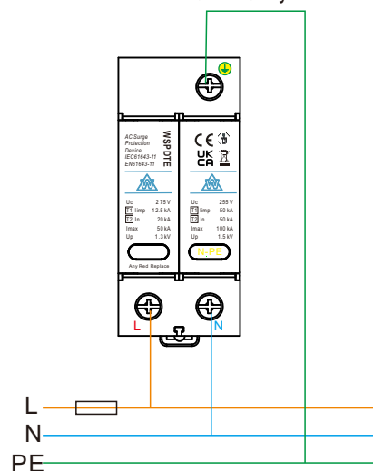
TN-S/ TN-C-S (PME) System
