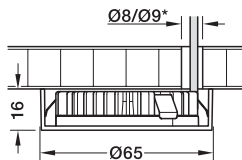
833.72.512, 833.72.513, 833.72.516 or 833.72.517 Round version bezel
