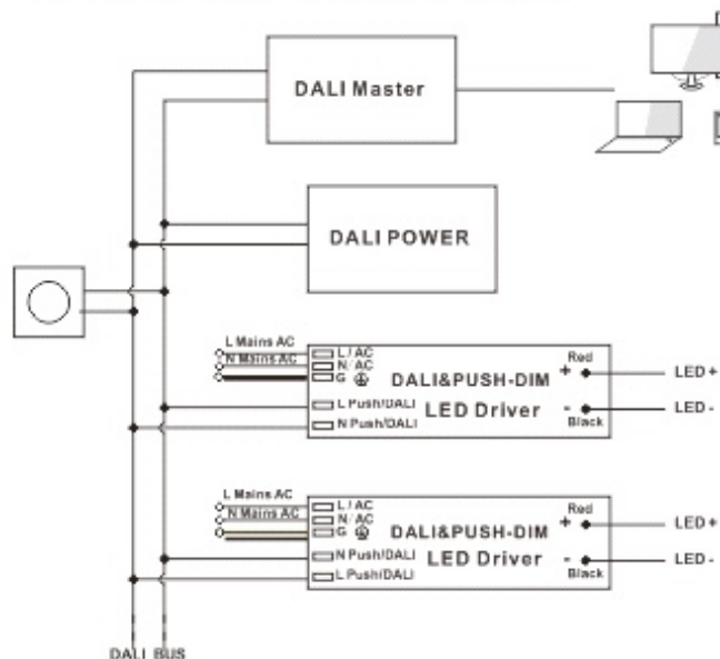
PC+DALI Master+DIMMER
