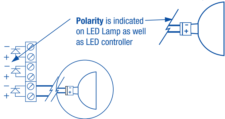
CORRECT Installation
