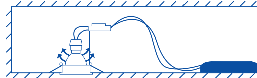
CORRECT Installation
