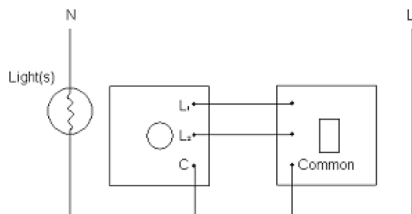
Figure 3 Using a 2-way Dimmerswitch
