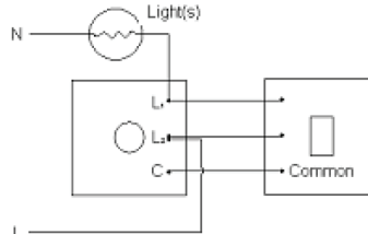
Figure 4 Using a 2-way Dimmerswitch
